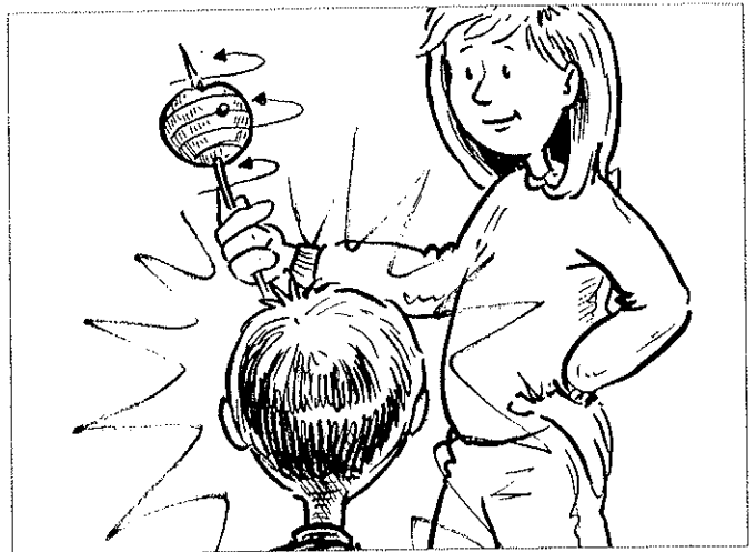
Earth's orbit around the sun.
